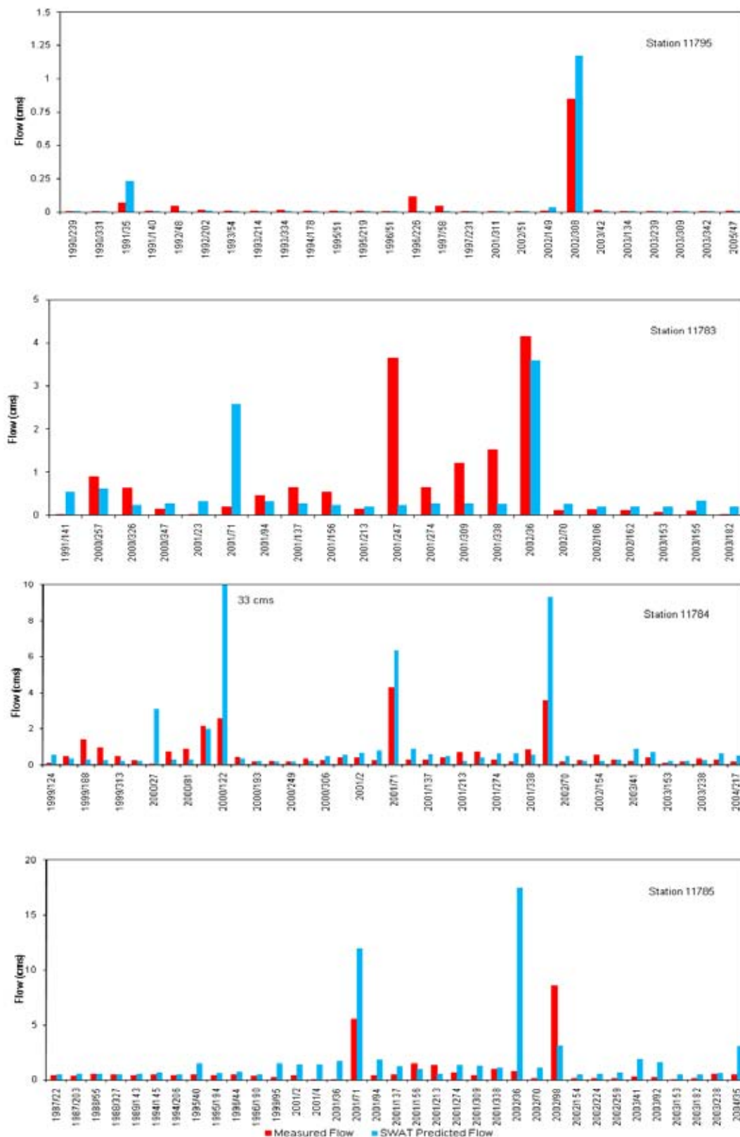
Figure 3-5 Comparison between the model-predicted flows and measured flows at four water quality monitoring stations
