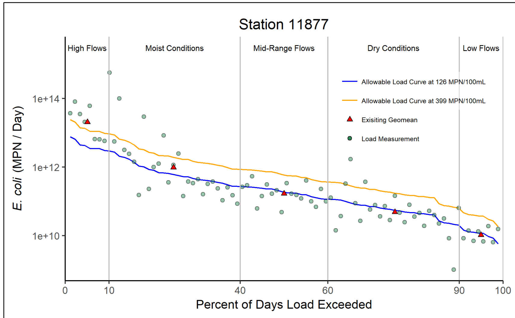
Figure 8. Load duration curve at Station 11877 Navasota River at US 79 (AU 1209_05) for the period of January 2000 through February 2016
