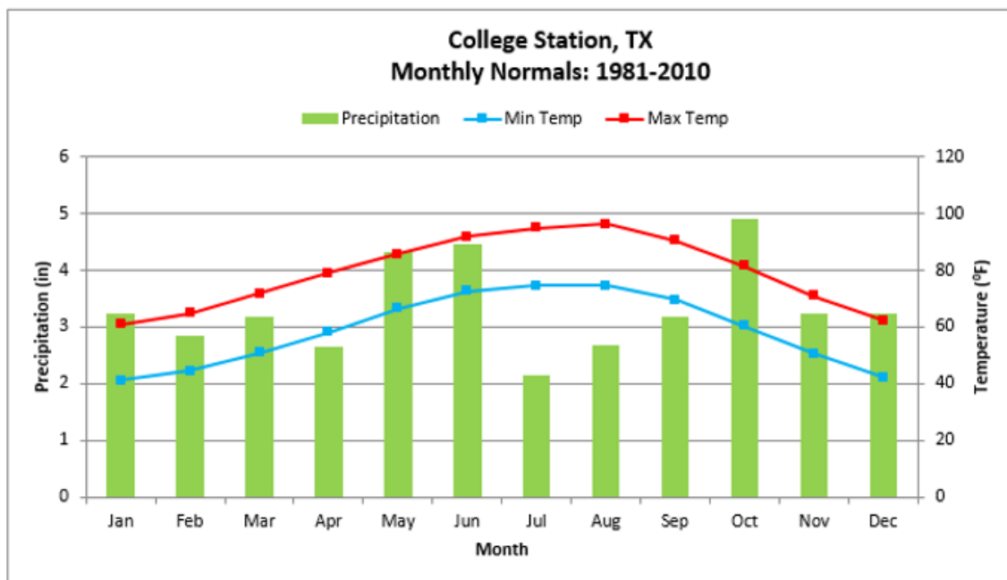
Figure 2. Average minimum and maximum air temperatures and total precipitation by month over 1981-2010 for the College Station area in the Navasota River below Lake Limestone watershed
