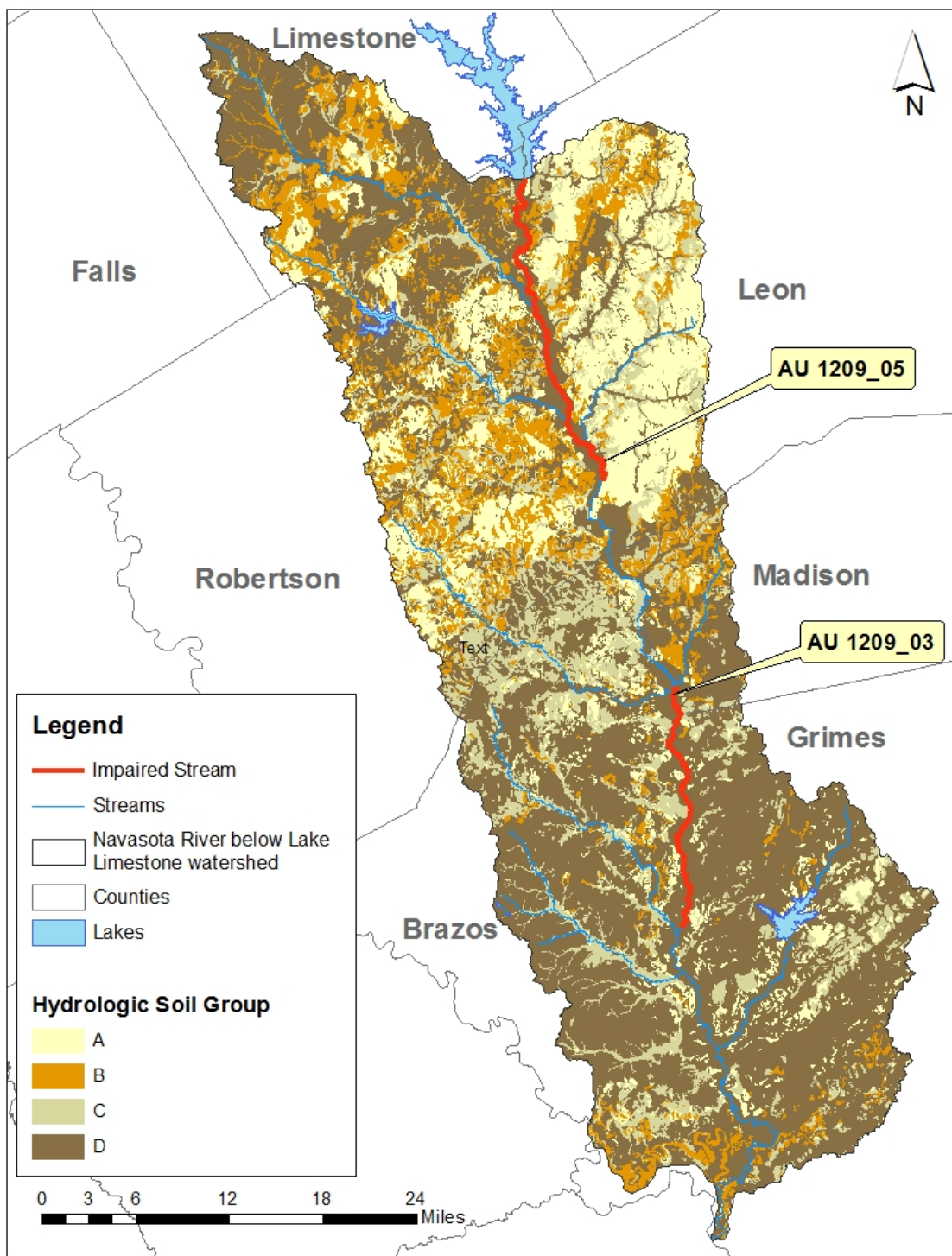
Figure 6. Hydrologic Soil Groups for the Navasota River below Lake Limestone
