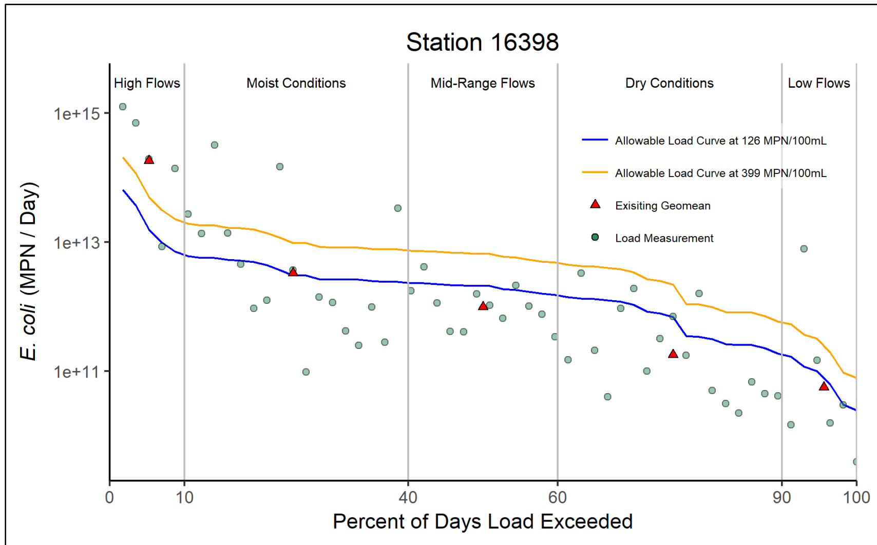
Figure 7. Load duration curve at Station 16398 Navasota River at Grimes (AU 1209_03) for the period of September 2001 through February 2016
